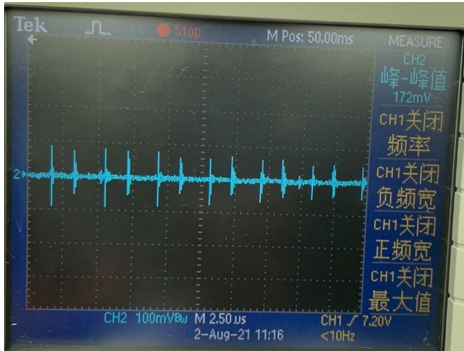
Noise ( V_{IN} = 48V , I_O = 6A , 5 ~ 20MHz bandwidth)
