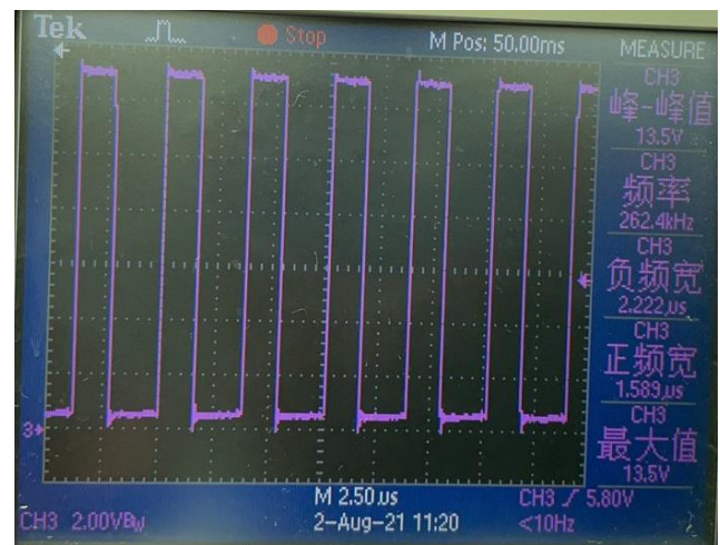
PWM waveform
